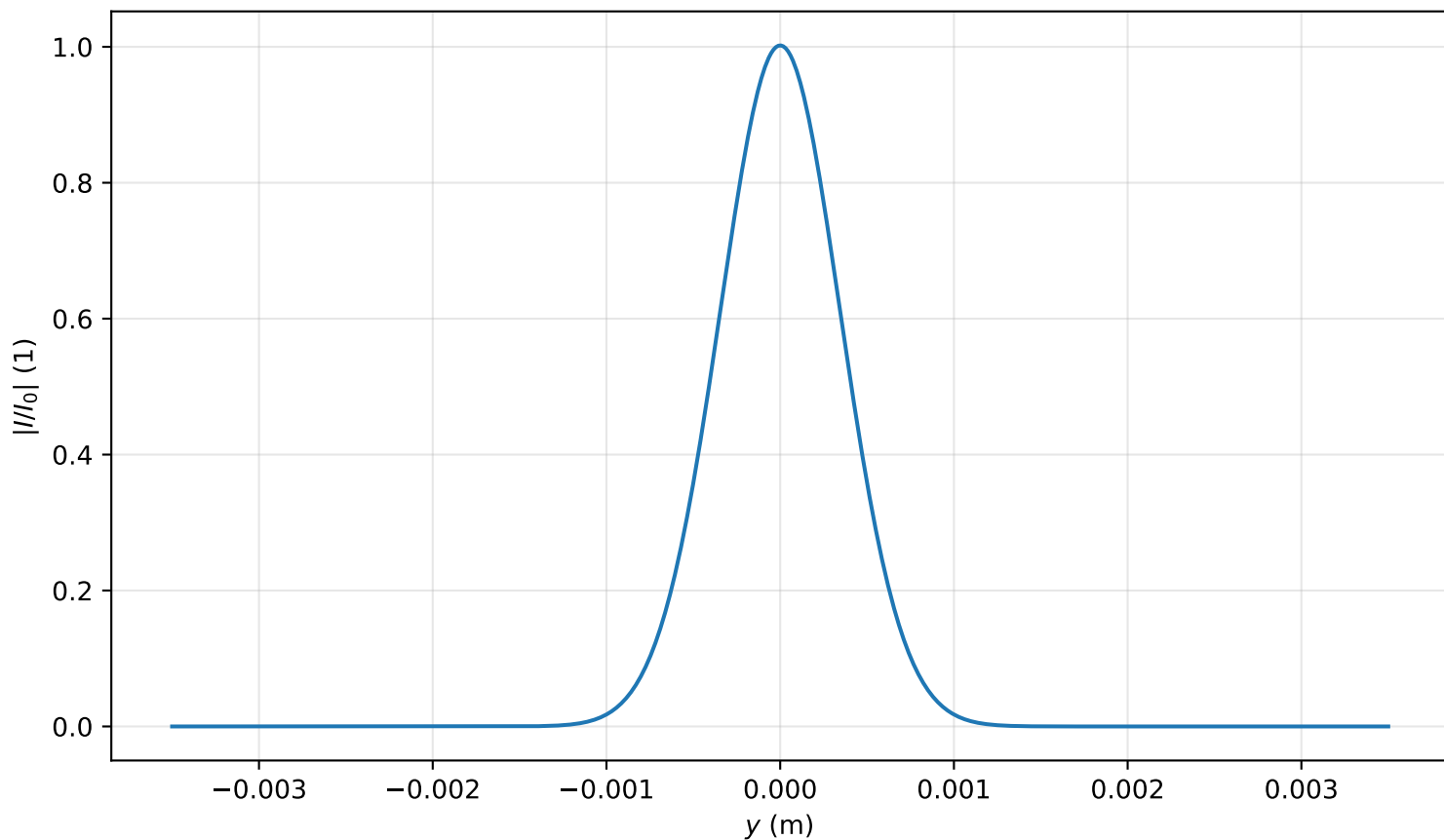
Intensity profile I(x=0, y, z=0.239)/I_0 , P_{in}=0.3P_{cr} , artificial time
